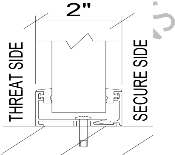
(Sill Detail Shown Above With Glazing Thickness 3/4" to 1 3/8")
